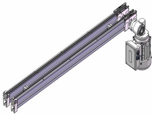
UTS1 Synchronous Belt UTS1 齿形带托盘输送线
