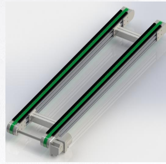
Synchronous toothed 同步齿形带型输送线 BTC07/BTC08
