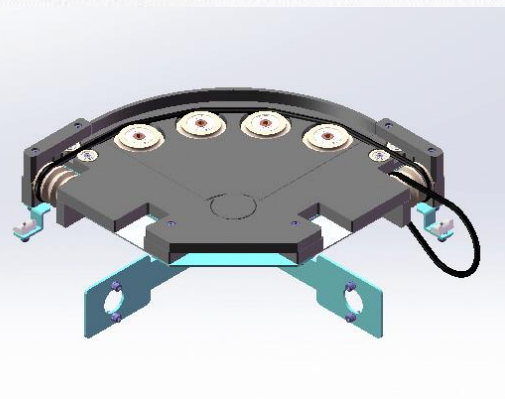
90° /180°Round Belt Curve 90°/180°圆皮带转弯
