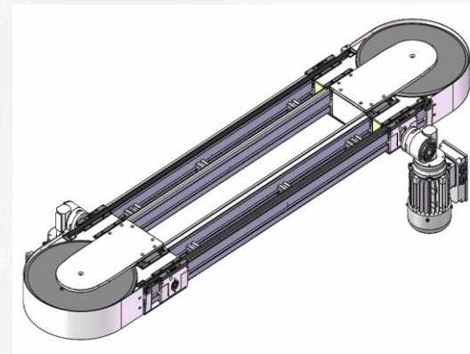
Circular Line UTS1齿形带环行线
