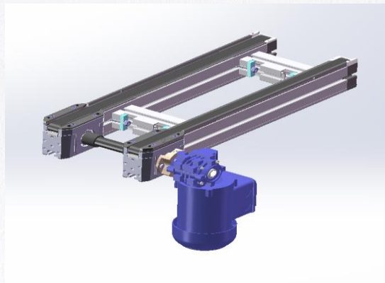
UTS2 TBC2 Tooth Belt Conveyor UTS2 齿形带托盘输送线
